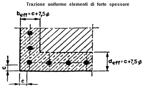
Fig. 4 - Area efficace
